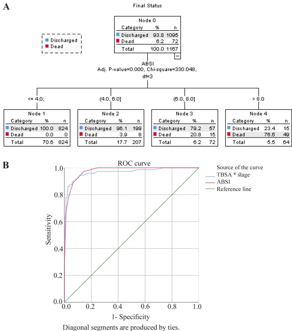
Figure 2. A) Decision tree extracted using CHAID analysis of the ABSI of the patients; Correct prediction in 98.6% of discharged cases, 68.1% of expired cases, and 96.7% overall prediction correctness. B) ROC curve evaluating sensitivity of ABSI (Area: 0.976, p < 0/001 ) and VI (TBSA*Stage) (Area: 0/967, p < 0/001 ) for prediction of death in this population.
